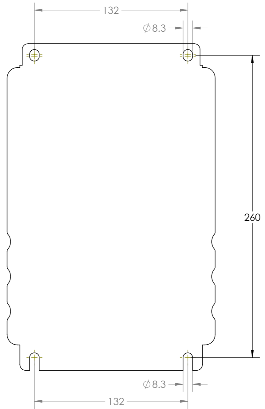
Transvend - Mount template dimensions - 2 Litre water heater
