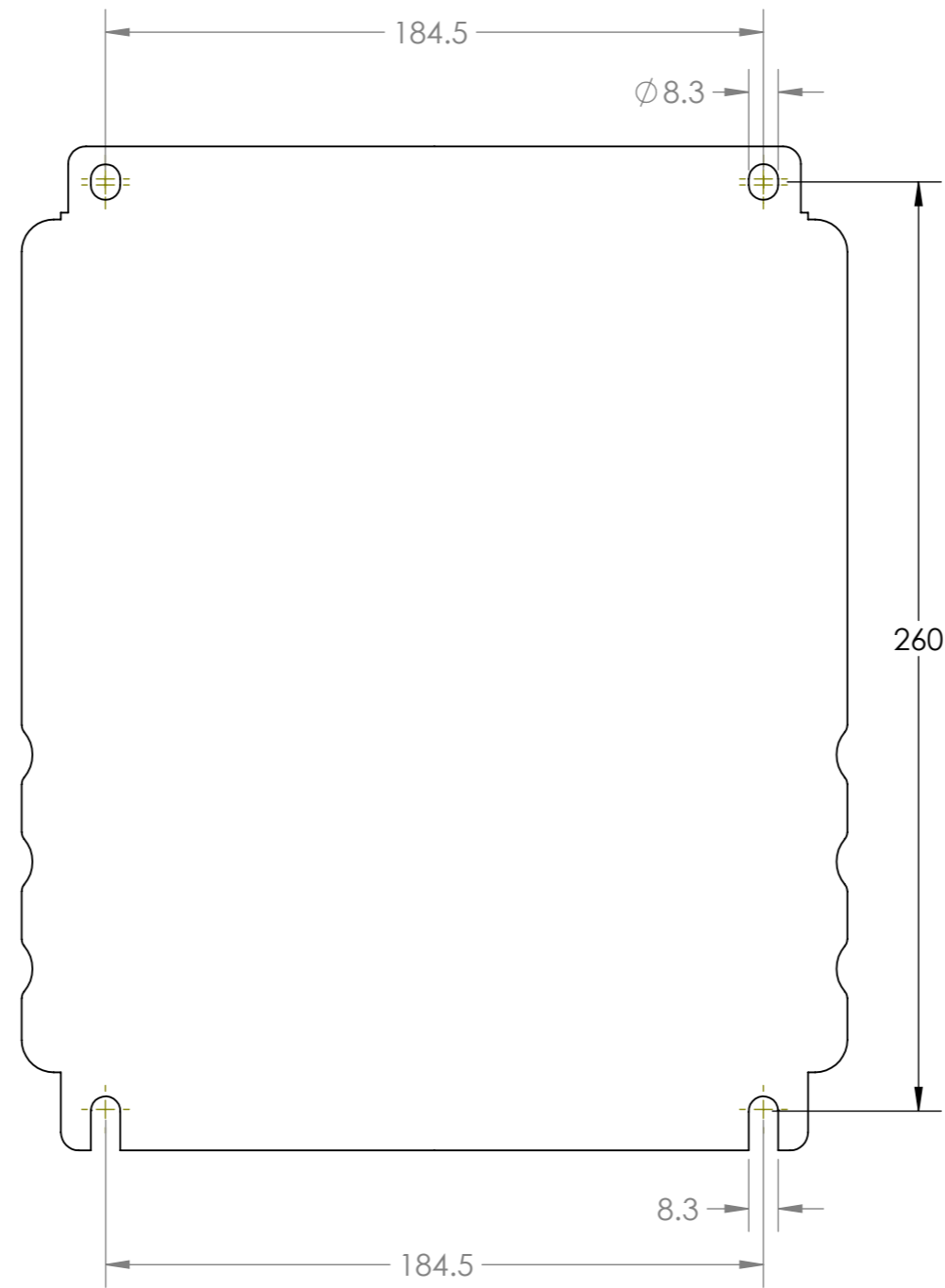
Transvend - Mount template dimensions - 3 Litre water heater
