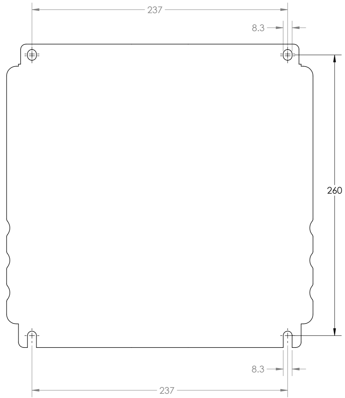
Transvend - Mount template dimensions - 4 Litre water heater
